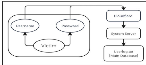
Fig.4. Backend working of QCJacking
