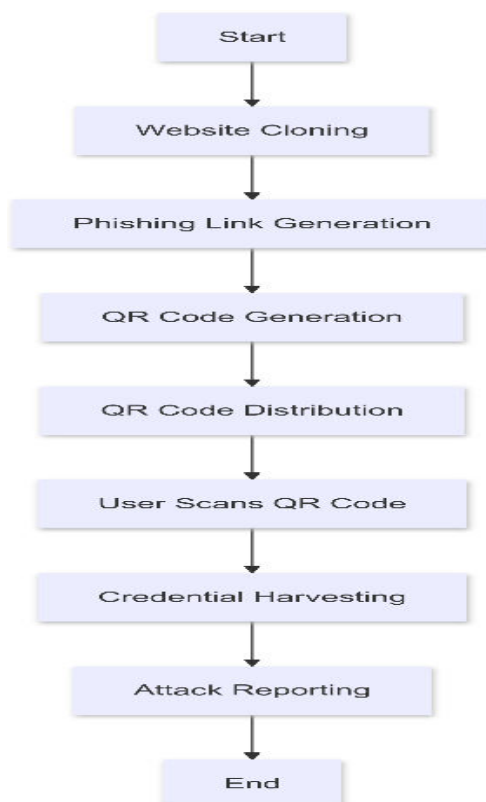
Fig.1. Block Diagram of QC-Jacking
